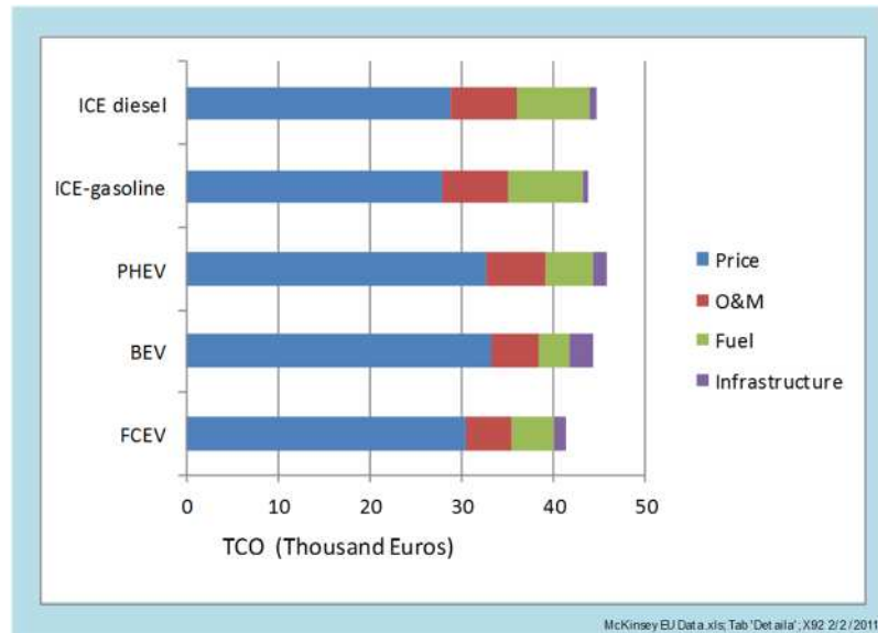
Figure 1. McKinsey estimate of vehicle total cost of ownership (TCO) in 2050 for SUV-sized vehicles
